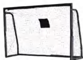
XY-G182TG Size:182x120x60cm XY-G220TG Size:220x170x80cm XY-G300TG Size:300x200x120cm Tube size: \phi 50 \times 0.9\text{mm} & \phi 38 \times 0.7\text{mm}
