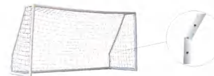
XY-S365C (Upgrade) Size: 365x182x120cm Tube size: \Phi 68 \times 1.8\text{mm} & \Phi 40 \times 1.3\text{mm}
