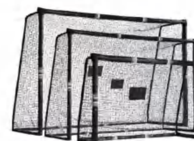
XY-G182PM Size: 180*120*60cm XY-G240PM Size: 240*160*85cm XY-G300PM Size: 300*200*120cm Tube size: \Phi 32 \times 0.8\text{mm}
