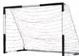
XY-G182E Size:182*120*60cm XY-G240E Size:240*160*80cm XY-G300E Size:300*200*120cm Tube size: \phi 50 \times 0.9\text{mm}
