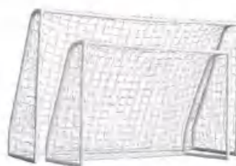
XY-S182B Size: 182*120*80cm XY-S245B Size: 245*155*90cm Tube size: \Phi 40 \times 1.3\text{mm} Material: UPVC tube, PP connection
